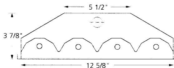
Hi-Bay End View
